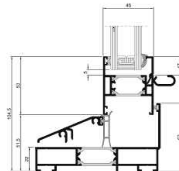
Cill Detail
