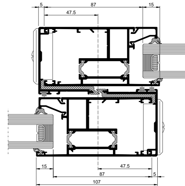
Interlock Detail
