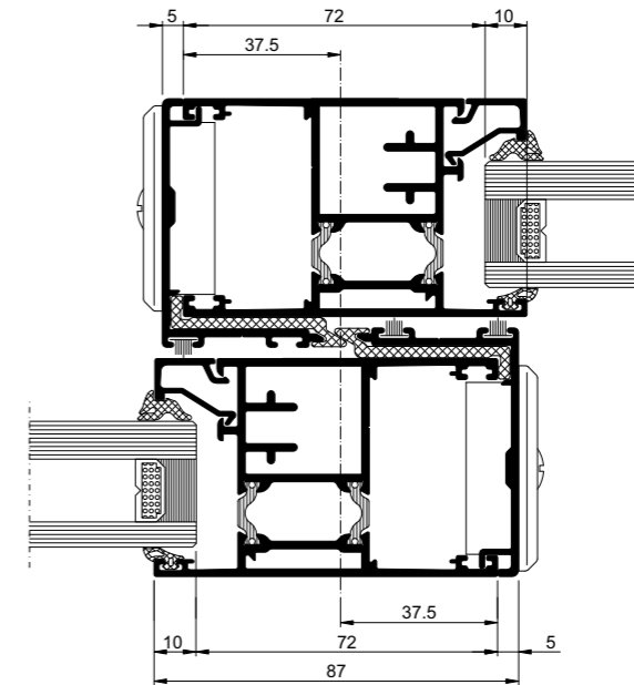
Interlock Detail
