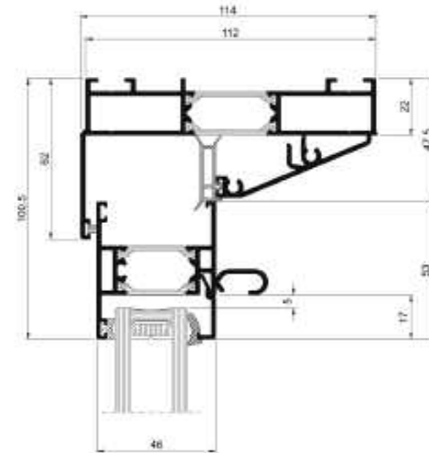
Head Detail
