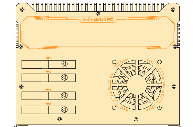
Rear Panel External I/O Mechanical Layout/Drawing
