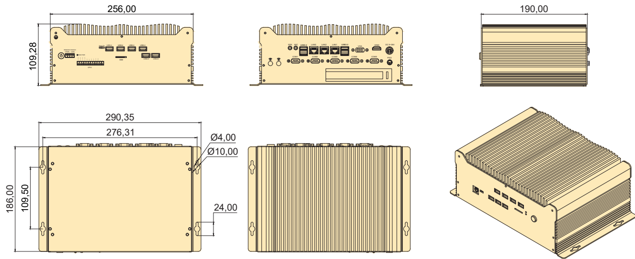
Front Panel External I/O Mechanical Layout/Drawing
