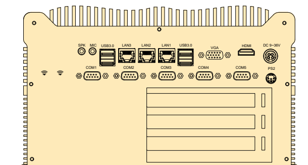
Rear Panel External I/O Mechanical Layout/Drawing
