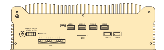
Front Panel External I/O Mechanical Layout/Drawing
