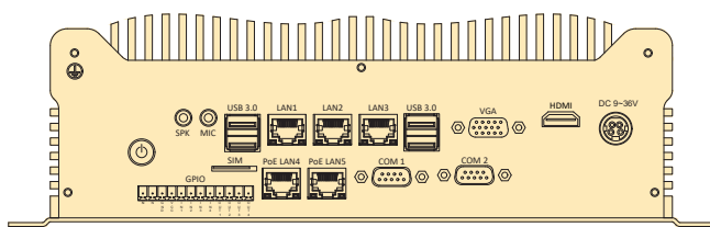
Front Panel External I/O Mechanical Layout/Drawing
