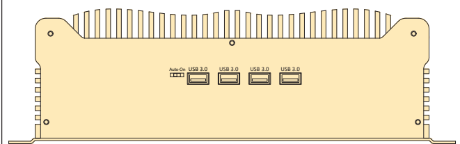
Rear Panel External I/O Mechanical Layout/Drawing
