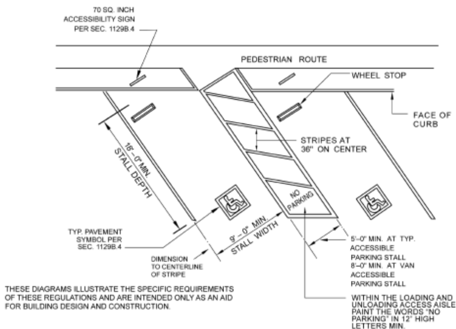
FIGURE 11B-18C—DIAGONAL PARKING STALLS
