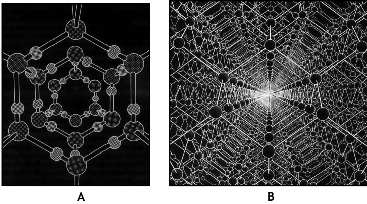
FIGURE 4-3. This schematic is believed to resemble the network structure of liquid water; however, scientists have been able to observe only a fraction of the network using current technologies. In view A , the large dark spheres representing oxygen atoms are connected to the smaller and lighter-shaded spheres representing hydrogen atoms. Hydrogen atoms are situated along the connecting hydrogen bonds. Water’s hydrogen-bonded network is difficult to depict at the scale of view B ; nonetheless, note the seemingly infinite matrix that exists among individual water molecules as hydrogen bonds (white lines) intersect oxygen atoms (black spheres). The network’s structural complexity, along with its hydrogen bond dynamics, may ultimately prove to be the key to water’s magic. Reprinted from Perspectives on Biogeochemistry . 13
