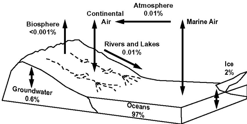
FIGURE 3-2. This simplified conceptual model of Earth’s hydrologic cycle shows the fraction of planetary water comprising each environmental compartment, which is presented as a percentage of the total water cycling through the system. Arrows indicate the major routes of water exchange among the various compartments; two-headed arrows indicate that water moves in both directions. According to the modern hydrologic regime, most of Earth’s water has been here since its formation, and the total volume of surface water has changed only slightly (e.g., due to large comet hits early in the planet’s history) over the last 4.5 billion years. While the assumptions underlying the modern hydrologic regime continue to be challenged and refined, there is no question that water’s global scale phase changes (e.g., solid to liquid to vapor) represent the primary mechanism by which solar radiation is converted into the energy that drives most planetary systems. The ultimate source of all freshwater is the oceans, where solar heating of seawater results in the evaporation that creates the clouds and sustains the winds for delivering global precipitation. Reprinted from Universal Water . 10
