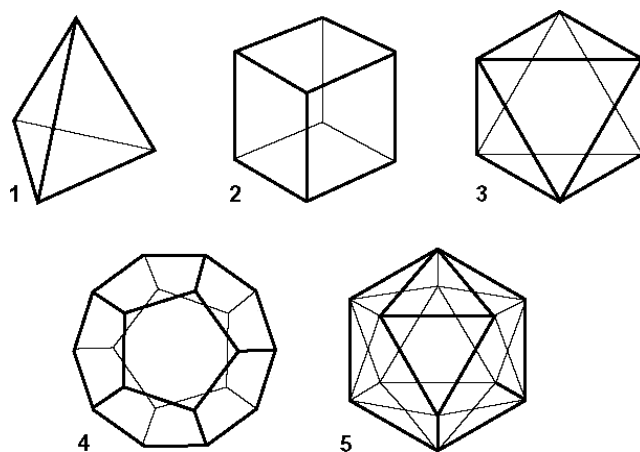
FIGURE 2-1. The five regular Platonic solids are the only angular three-dimensional geometries that are composed entirely of regular polygons and, when spun about their center vertex, create a sphere. The faces constitute the sides or exterior panels of the Platonic solids and are represented by a triangle, square, or pentagon. The edges are the straight lines that outline each of the faces, whereas the vertices are the points where two or more edges converge. The solids include a tetrahedron (1), a cube (2), an octahedron (3), a dodecahedron (4), and an icosahedron (5). Reprinted from Universal Water . 12
