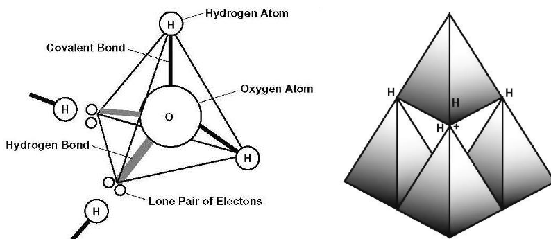
FIGURE 4-2. The schematic on the left represents the simplest unit of water's hydrogen bonded network. The large oxygen atom serves as the center vertex of a tetrahedron, while the smaller hydrogen atoms serve as its four outer vertices. Two of the hydrogen atoms are covalently bonded to the oxygen atom, comprising the individual water molecule ( \text{H}_2\text{O} ). Water molecules are hydrogen-bonded to each other via two pairs of electrons associated with each oxygen atom. These electron pairs attract two hydrogen atoms (each donated by a different neighboring water molecule) in forming a tetrahedron composed of one oxygen atom and four hydrogen atoms. Covalent bonds (thick black lines) create a water molecule by linking atoms together, whereas hydrogen bonds (thick gray lines) create a water network by linking molecules together. The schematic on the right is composed of four hydrogen-bonded water molecules. Linking water molecules together via different geometric arrangements creates a wide variety of water clusters. Reprinted from Universal Water . 6
