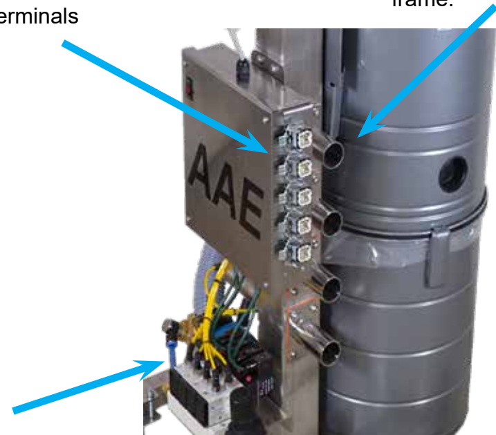
Fully assembled pneumatic manifold.
