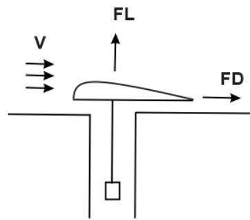
Figure 2 - Drag device (from Windmills in the Light of Modern Research )
