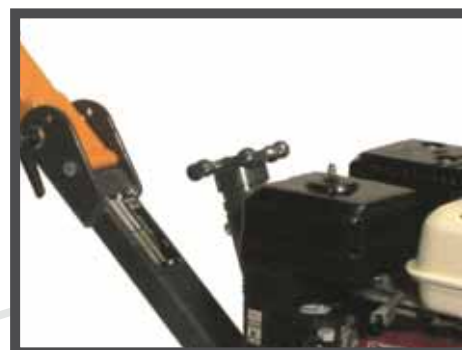
'SCREW PITCH' FOR EASY BLADE ADJUSTMENT
