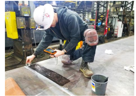
Ultrasonic Inspection
