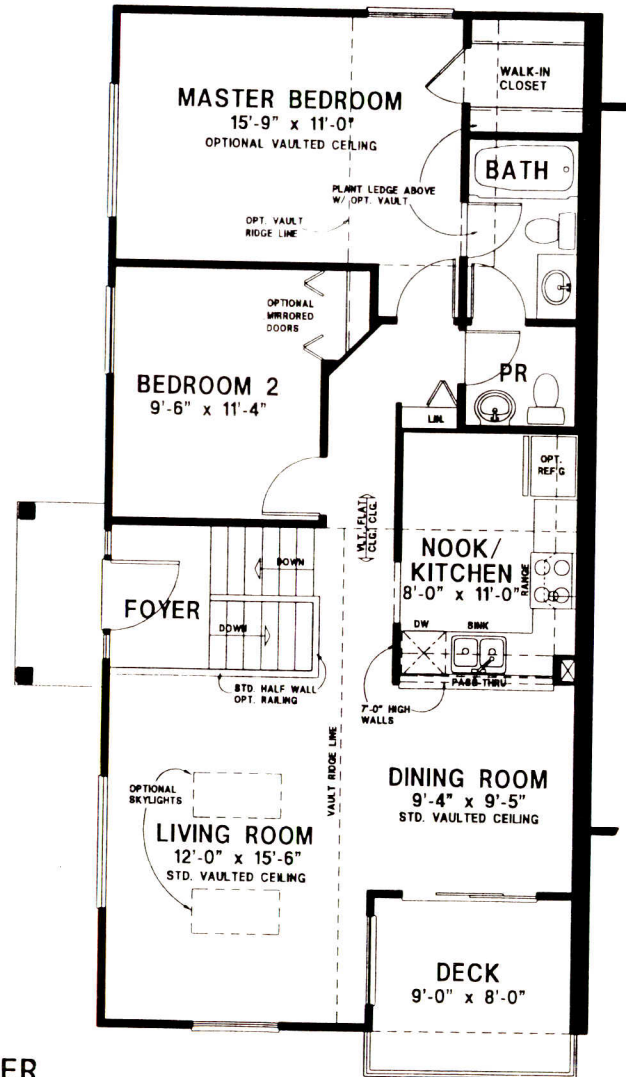
2 BED / 1 1/2 BATH UPPER LEVEL
