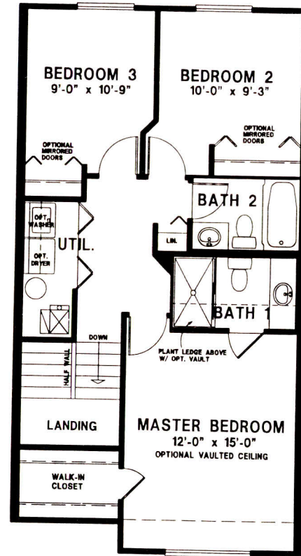
3 BED / 2 1/2 BATH UPPER LEVEL
