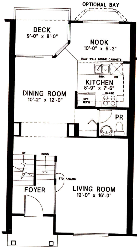
MIDDLE LEVEL THE DEERBORN
