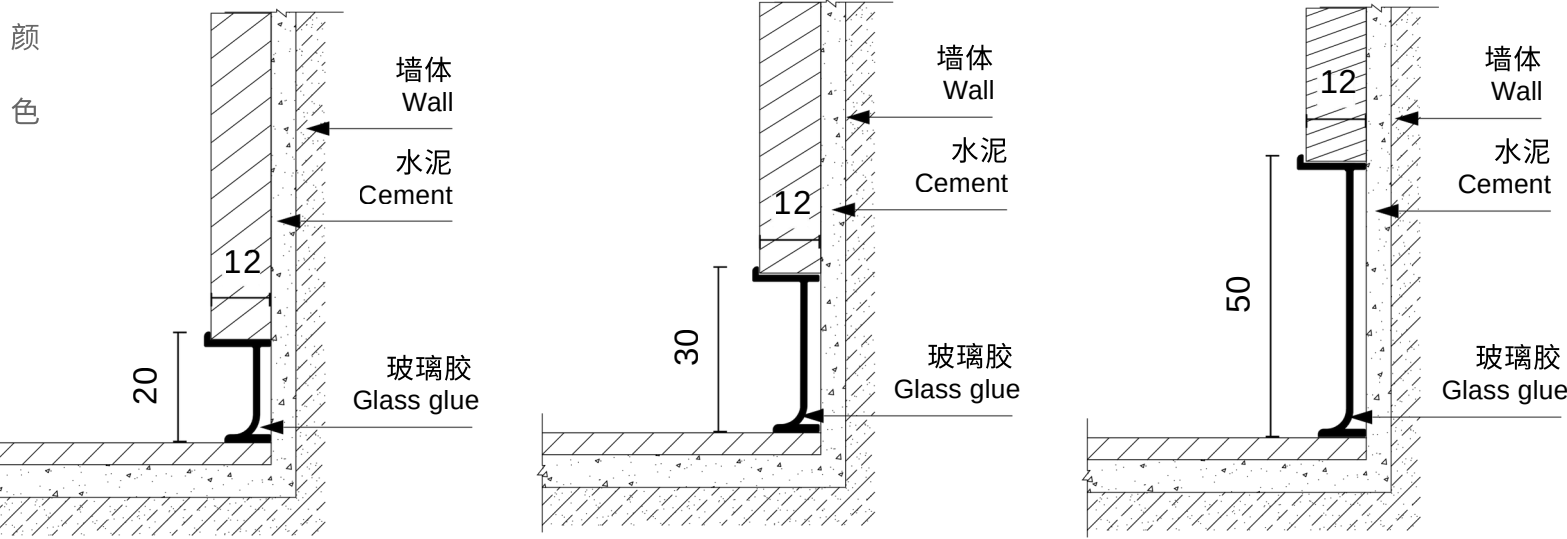
产品配件图 Product accessories drawing
