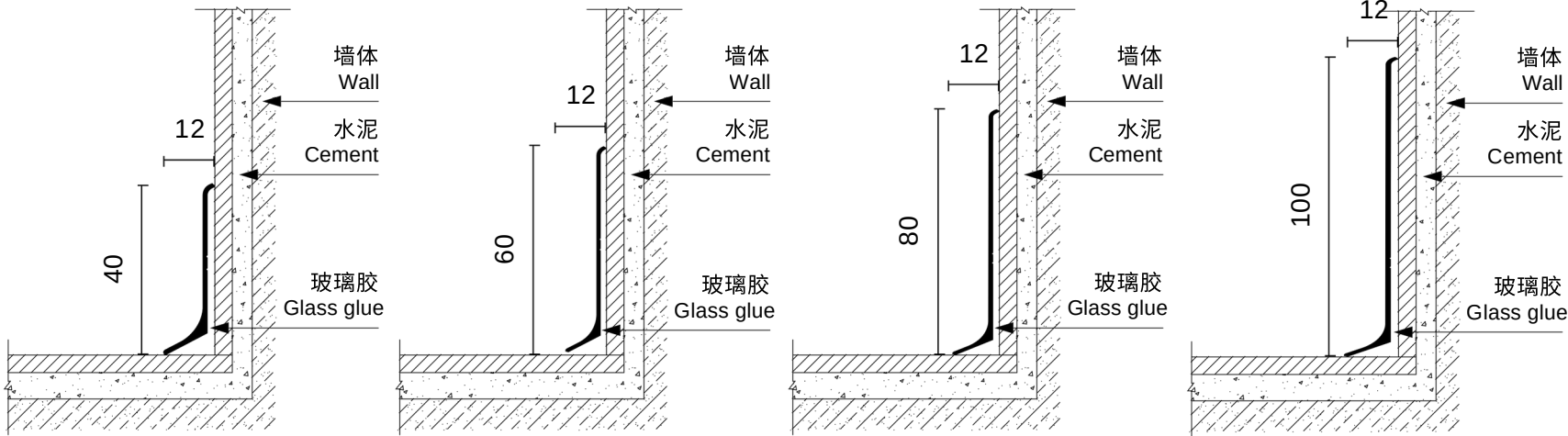
Product accessories drawing
