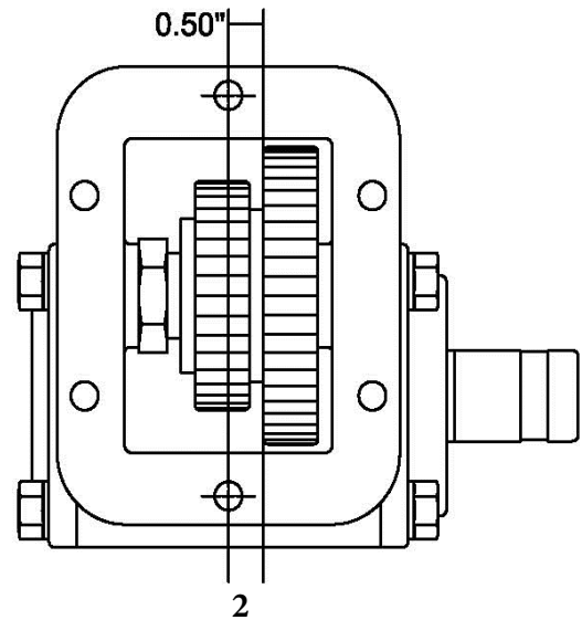
2 Right Side Output Rear Input Gear
