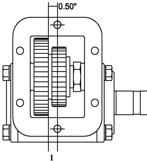
1 Right Side Output Forward Input Gear
