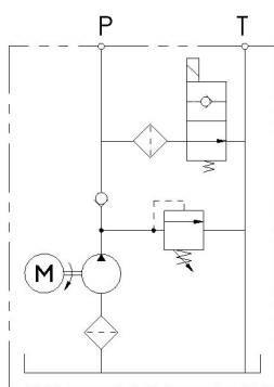
HYDRAULIC CIRCUIT A09 SINGLE ACTING NOT HOLDING
