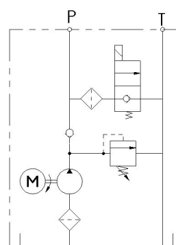
HYDRAULIC CIRCUIT A10 SINGLE ACTING
