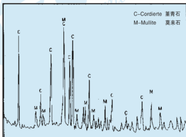
X-Ray Ciffraction of Cordierite-Mullite 堇青石-莫来石X衍射图谱
