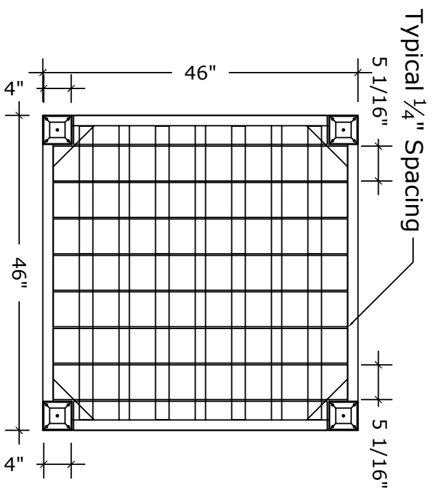
Typical Single Frame with Decking
