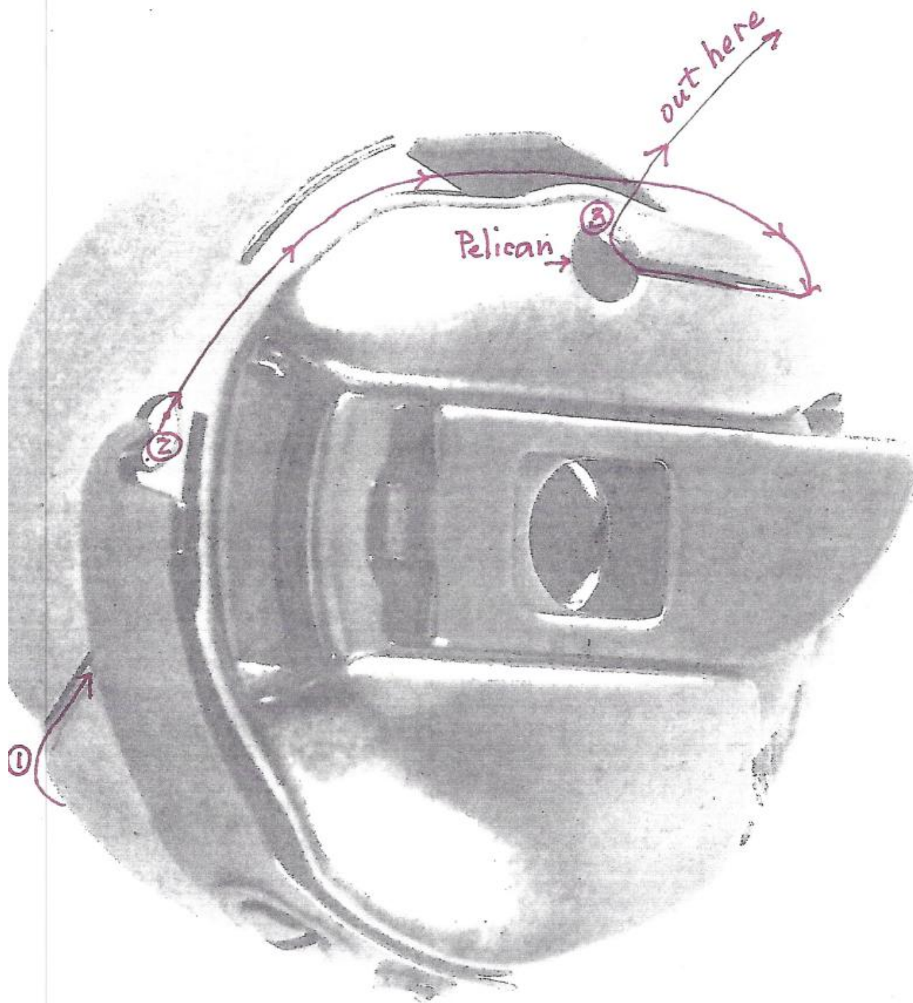
Bobbin Case Thread Path
