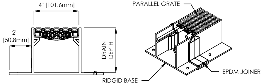
DECK DRAIN SECTION
