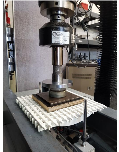
FIG. 2 COVER TEST SET-UP
