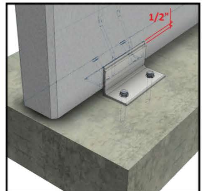
Concrete Tilt-Up Structures
