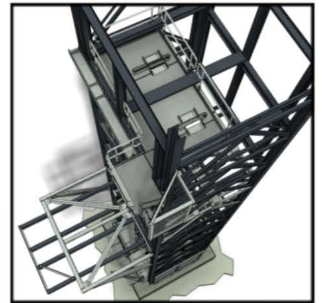
Head-frames / Shaft Steel & Safety Doors
