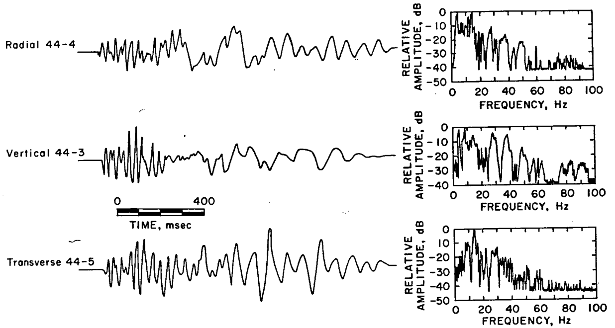
Figure 3.—Coal mine blast time histories and spectra measured at 2,287 ft.
