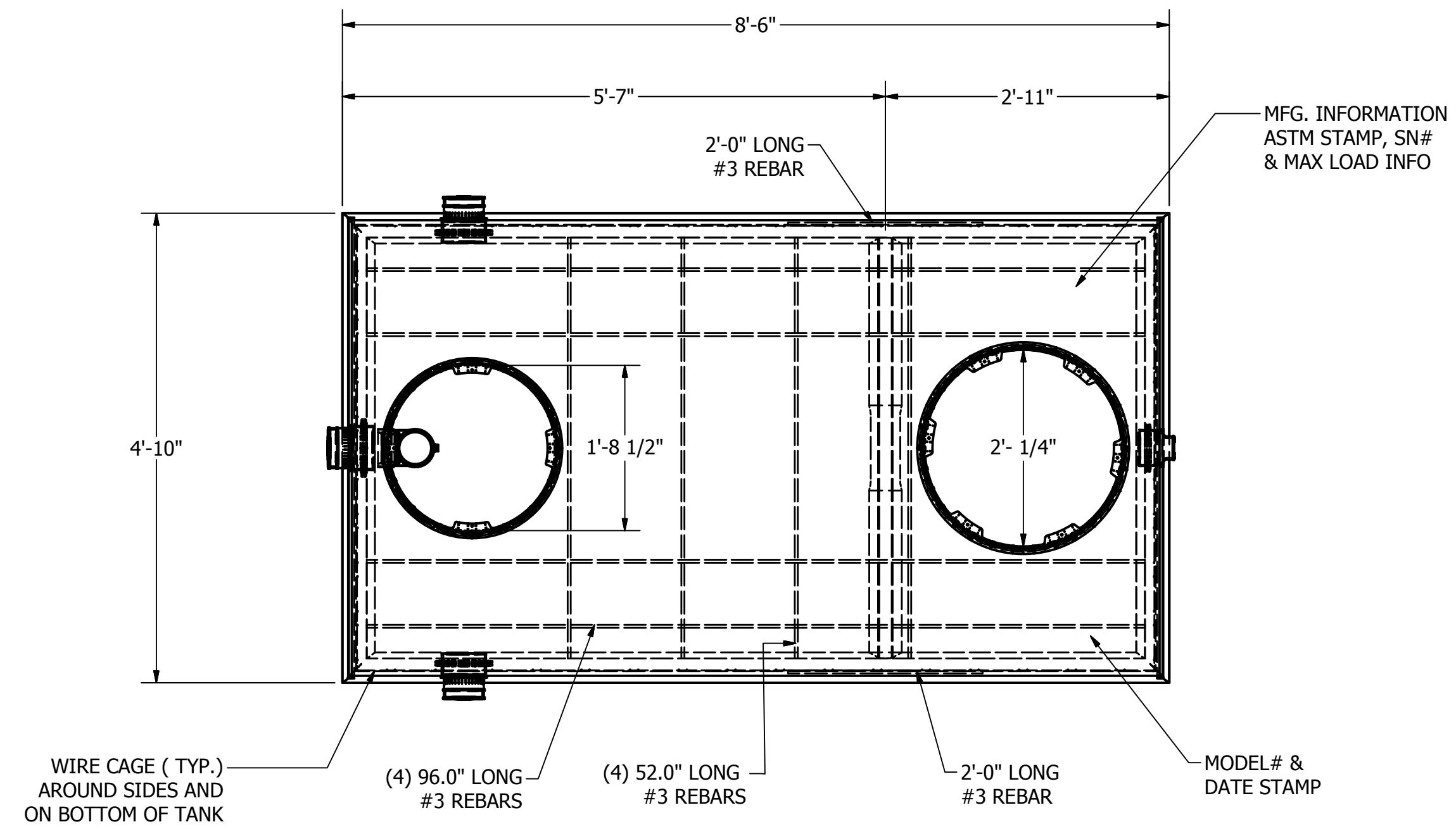
TOP VIEW ( RISER & SAFTEY COVERS REMOVED )
