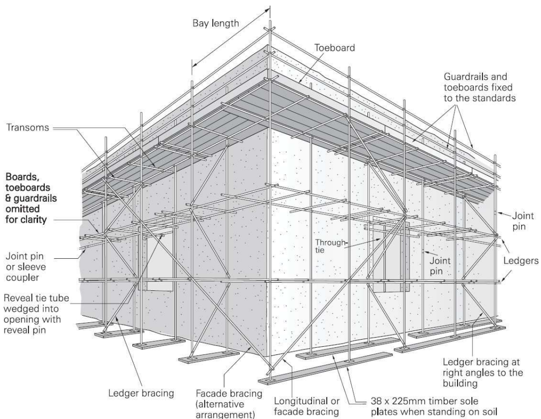
Figure Independent Tied Scaffold (note: single guardrails omitted from non-working lifts for clarity)
