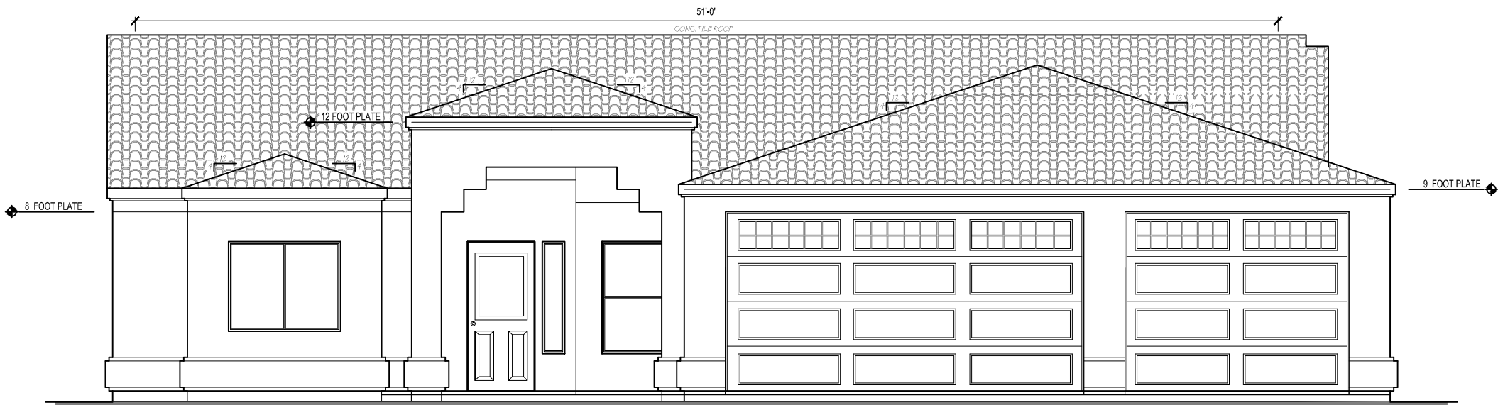
FLOOR PLAN & FRONT ELEVATION SCALE: 1/4" = 1'-0" 0' 1' 5' 10' 20'
