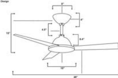
Size Chart Lantana Design
