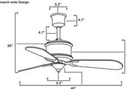
Size Chart Monarch wide Design
