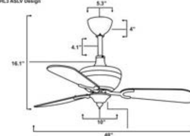
Size Chart SHL3 ASLV Design
