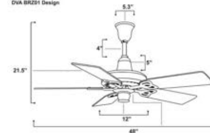
Size Chart DVA BRZ01 Design
