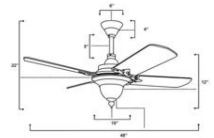
Size Chart Dynasty Design
