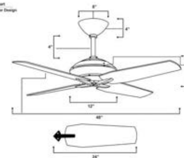
Size Chart Gladiator Design
