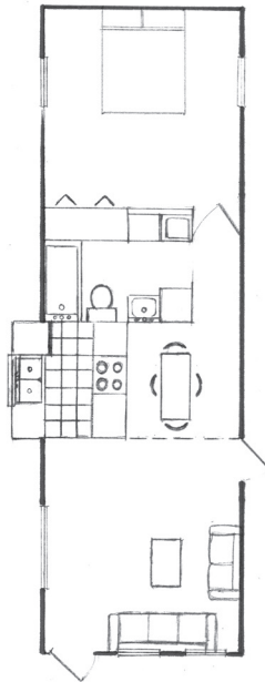
STICK BUILT CONSTRUCTION 12ft X 39ft Interior Front Porch
