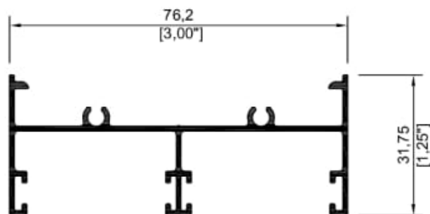
7826 Chambrana 3"
