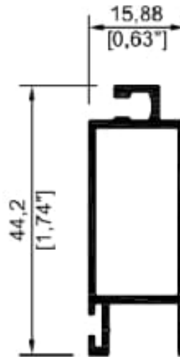
6534 Mosquitero vertical
