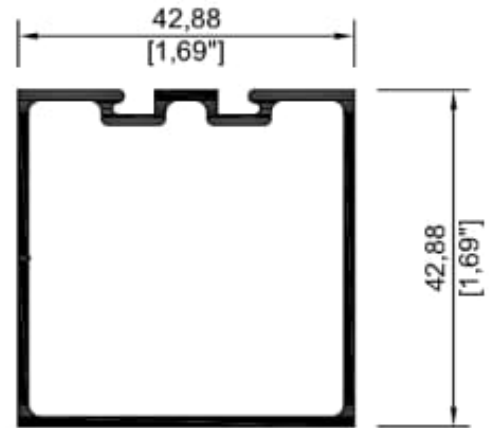
9184 Remate lateral
