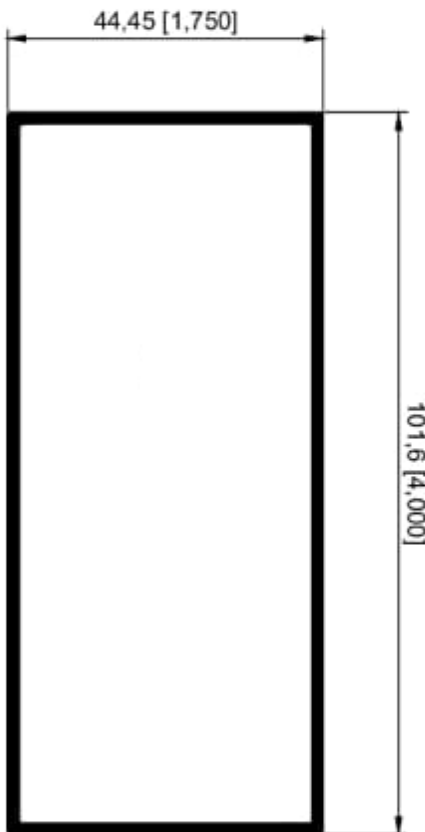
2520 Rectangular 4" x 1 3/4"
