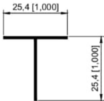
1613 Tee 1"
