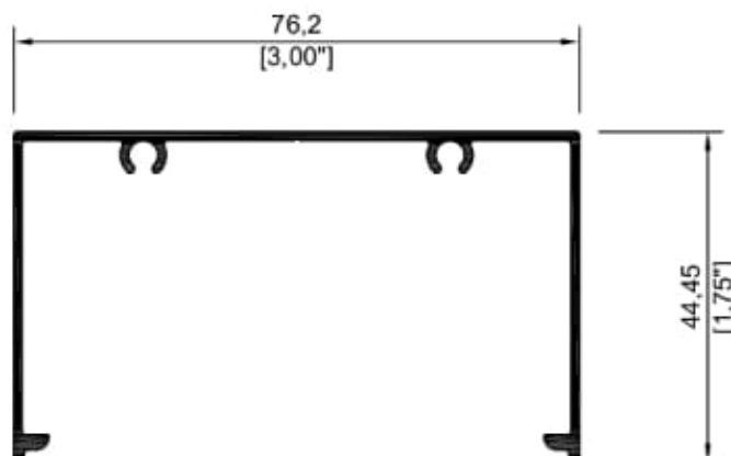
9114 Bolsa lisa 3"
