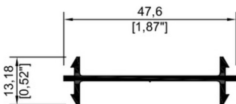
7792/4206 Mulion
