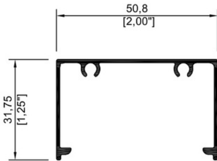
8591 Bolsa lisa 2"
