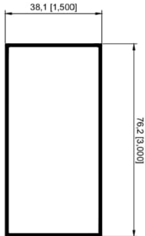
11084 Rectangular 3" x 1 1/2"
