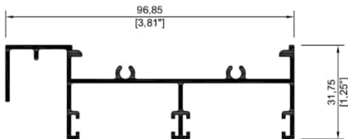
7862 Chambrana mosquitero 3"
