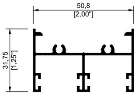
7518 Chambrana 2"
