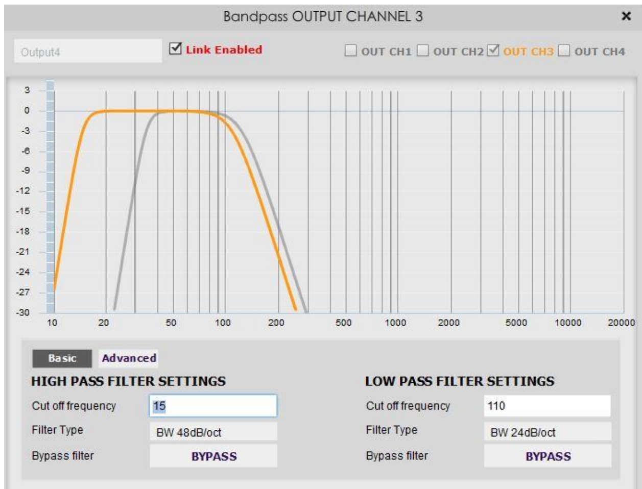
Diagram 11. Multiple subwoofer crossovers with high and low pass filter settings
