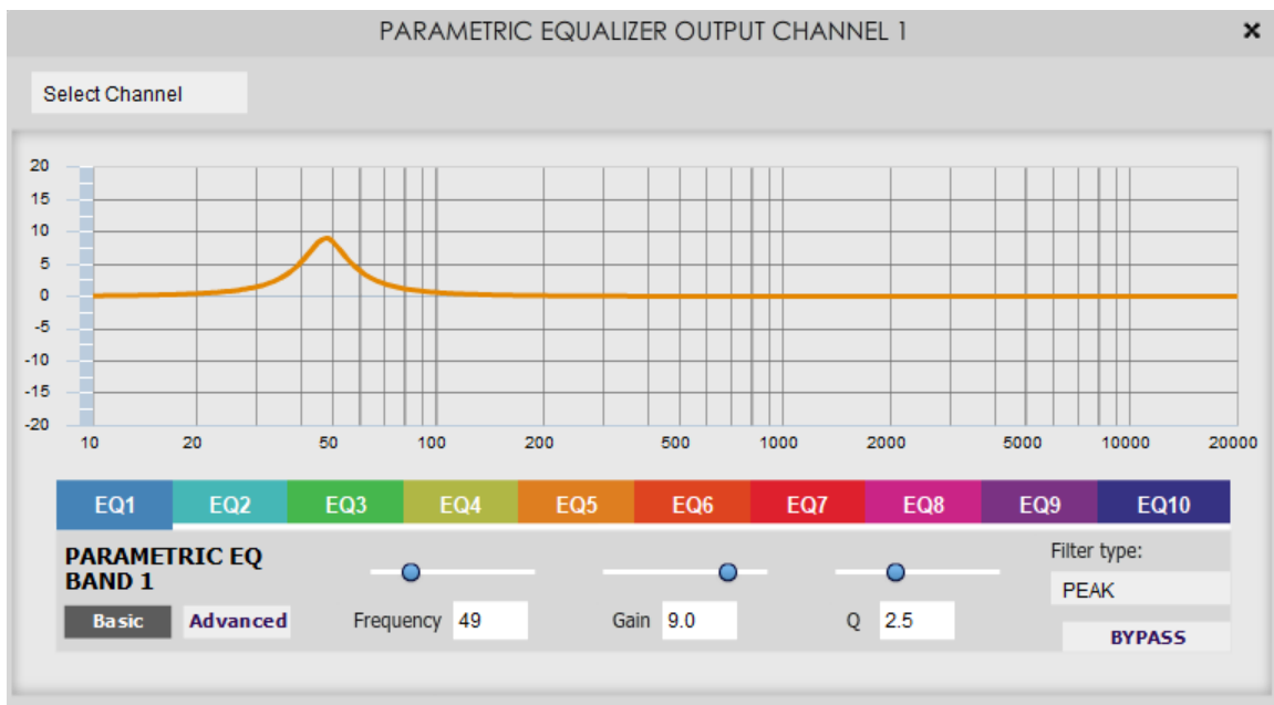
Diagram 19. Example of a tune-to-taste peak filter overlay used for adding some “punch”
