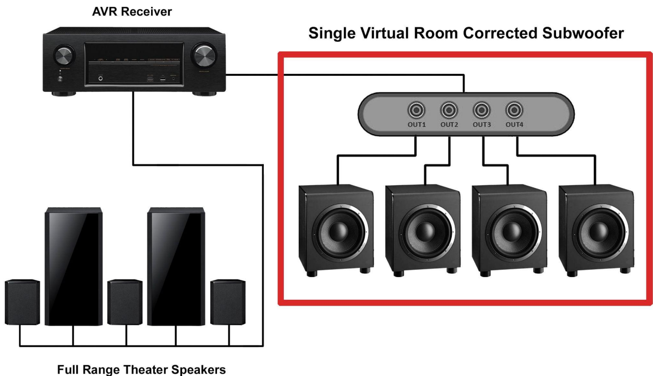
Diagram 1. Home theater with single virtual room corrected subwoofer
