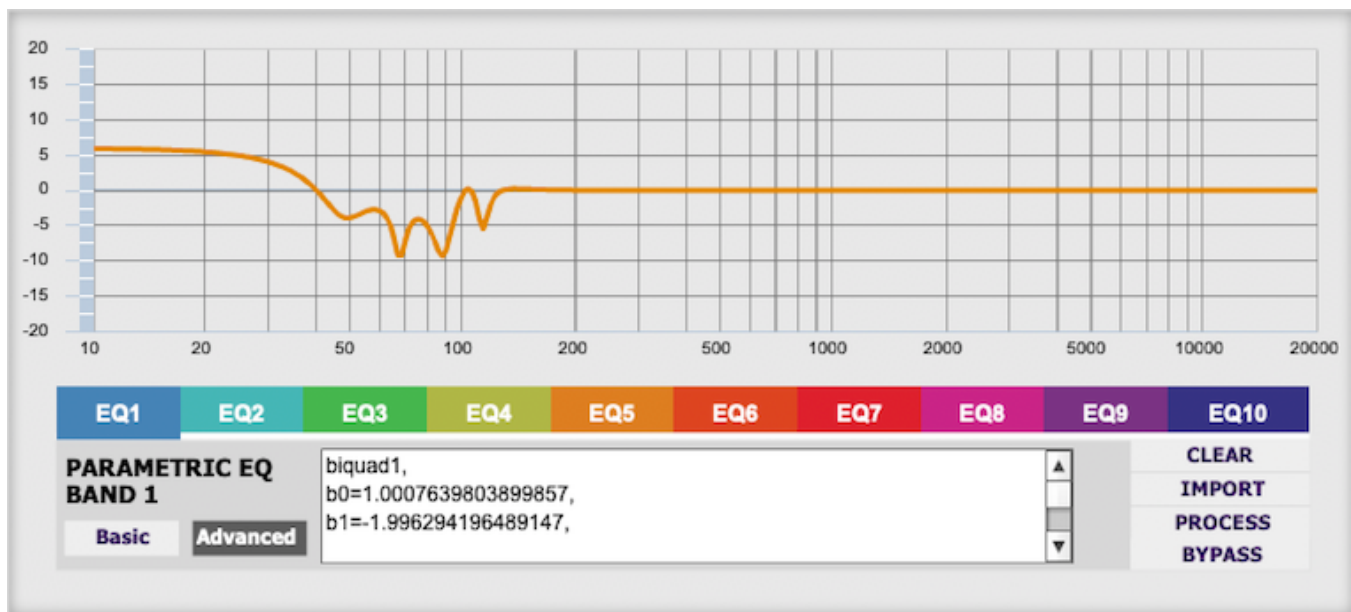
Diagram 17. Inverse filter downloaded and displayed in the miniDSP plug-in
