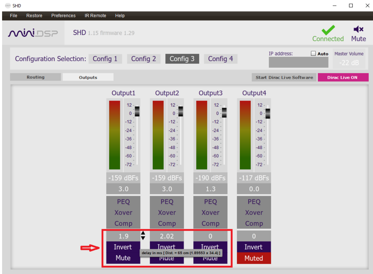
Diagram 10. Inserting time delay for coincident time of arrival
