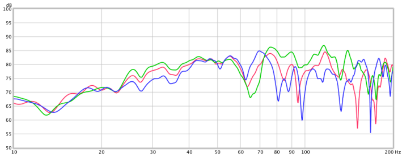
Diagram 12. Three subwoofer relative amplitude overlay plot
