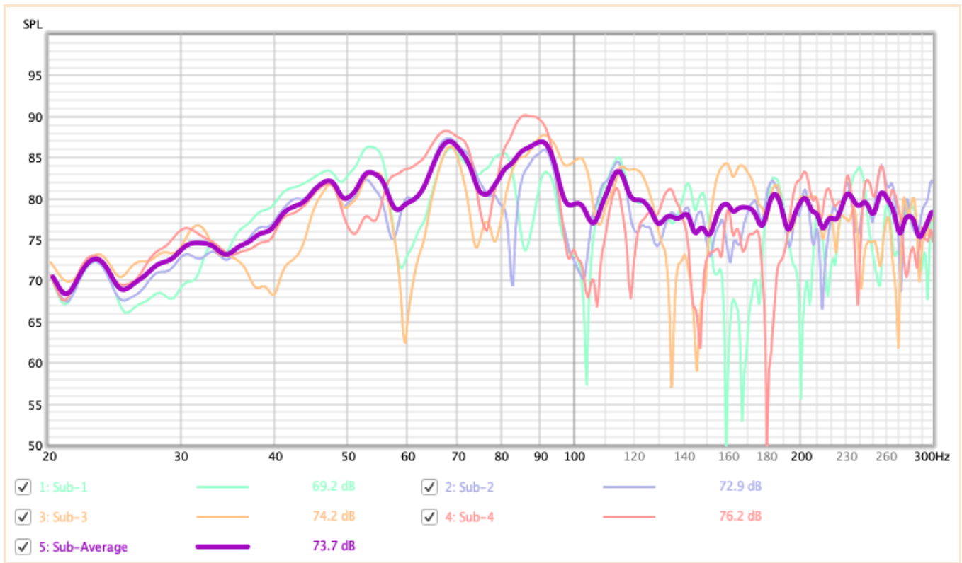
Diagram 14. Averaged multi-subwoofer room measurements
