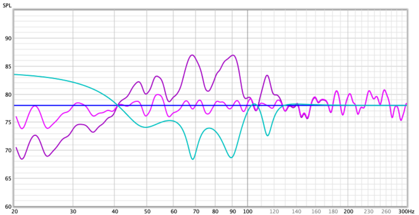
Diagram 16. Measured (purple), predicted (pink) and calculated inverse filter (turquoise) responses
