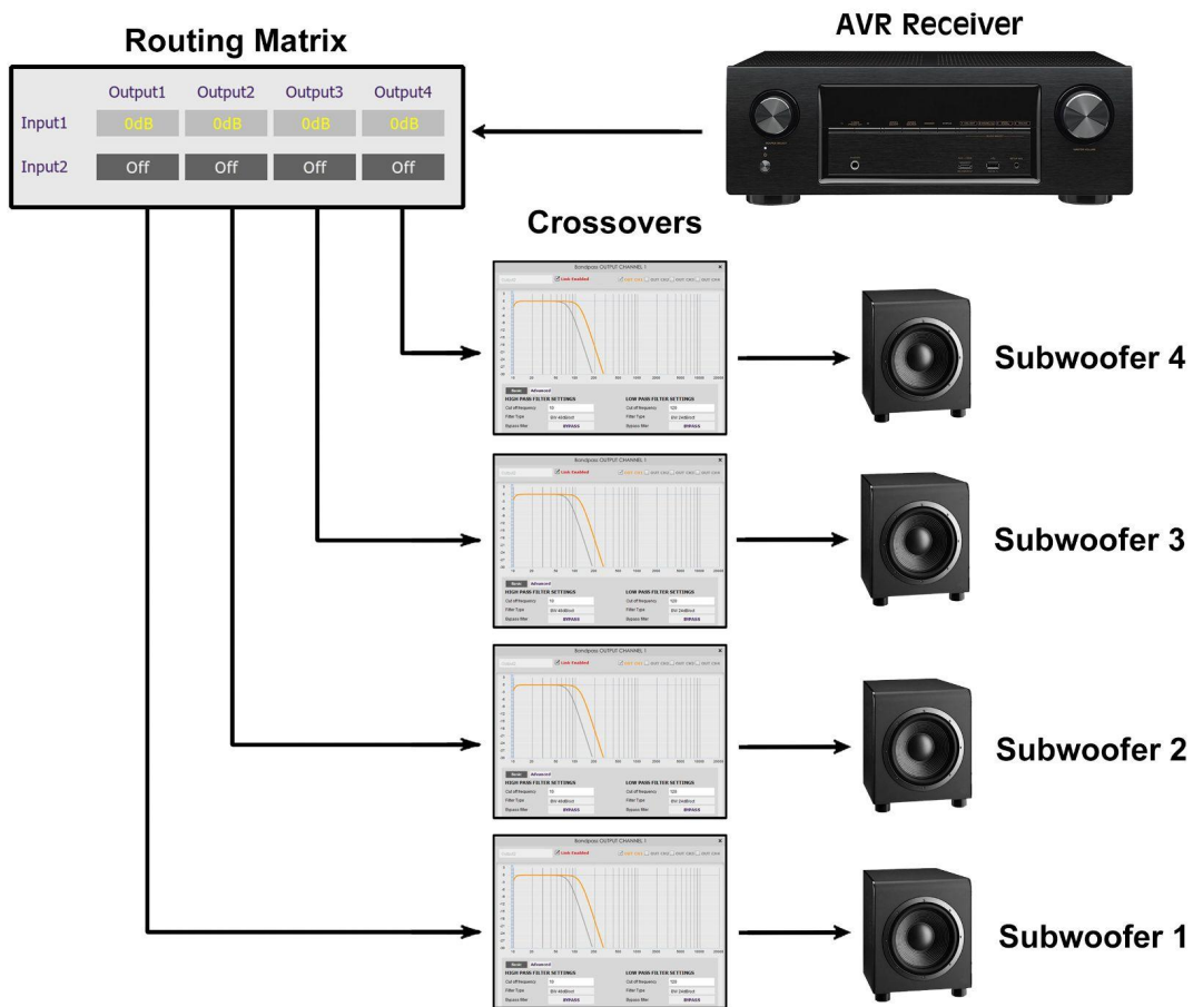
Diagram 4. Signal flow through the miniDSP showing routing, crossover and parametric equalization (PEQ)
