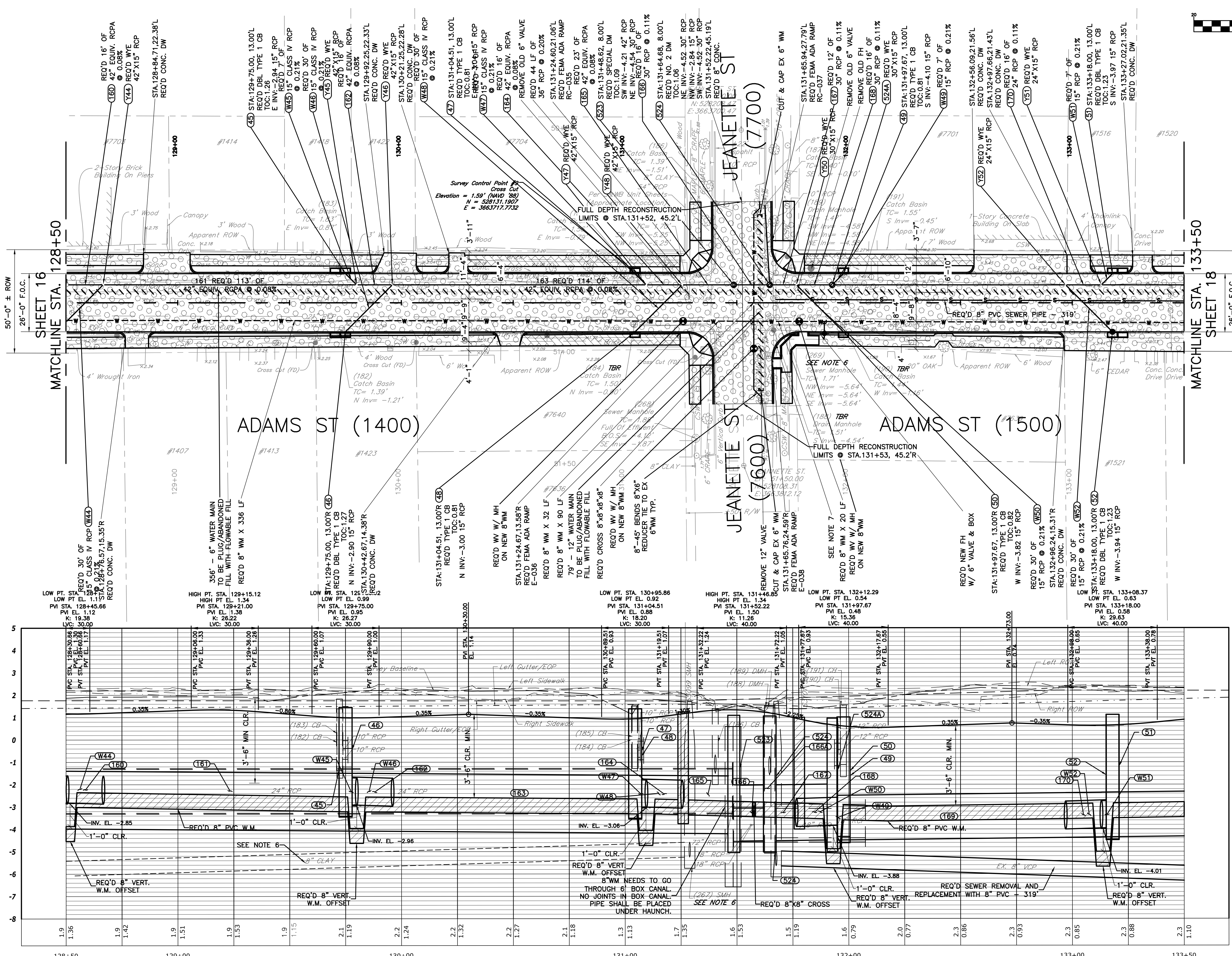
ADAMS STREET (STA: 128+50.00 to STA: 133+50.00) SCALE: 1"=20' HORIZ. / 1"=2' VERT.
