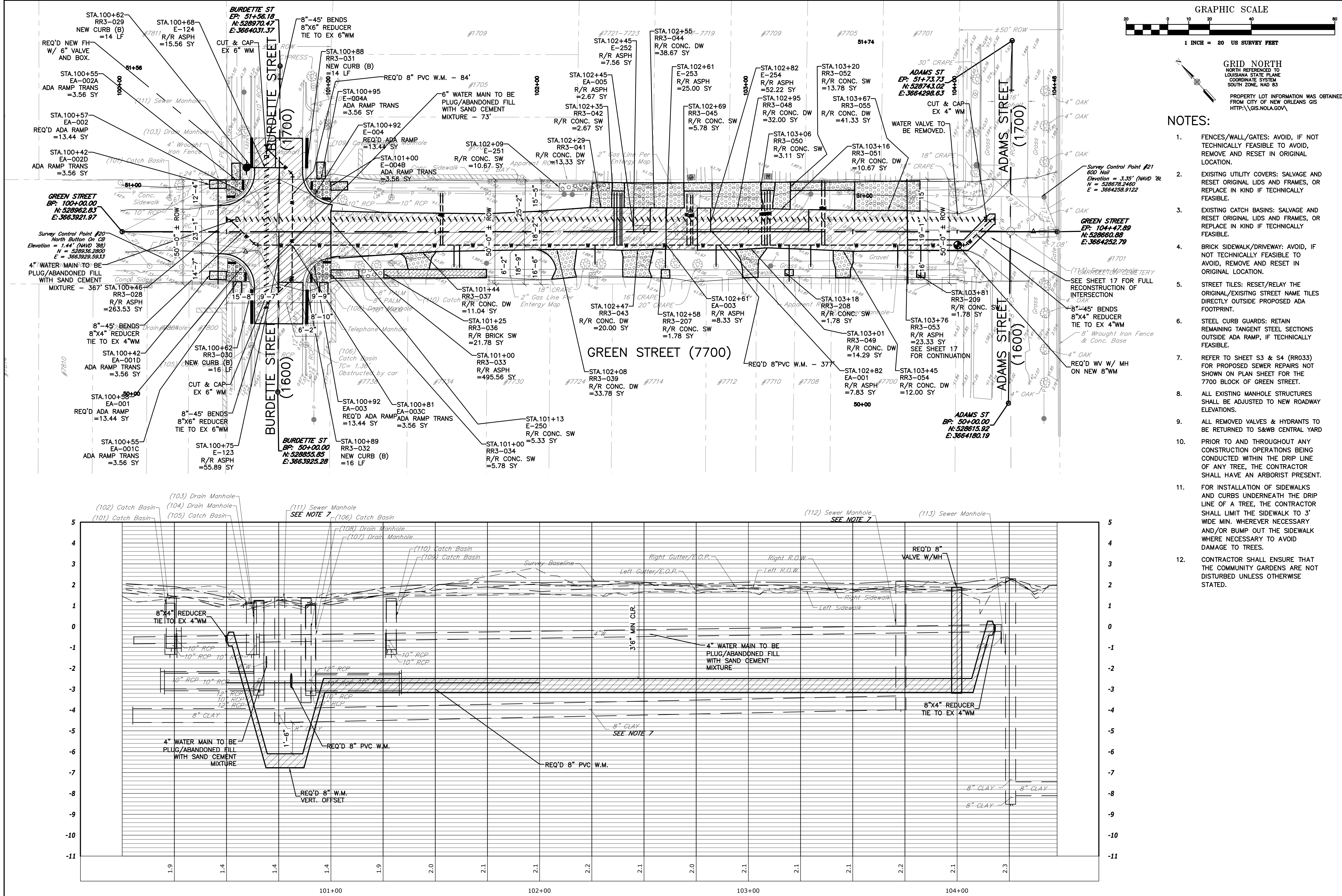
GREEN STREET (STA: 100+00.00 TO STA: 104+47.89) SCALE: 1"=20' HORZ. / 1"=2' VERT.
