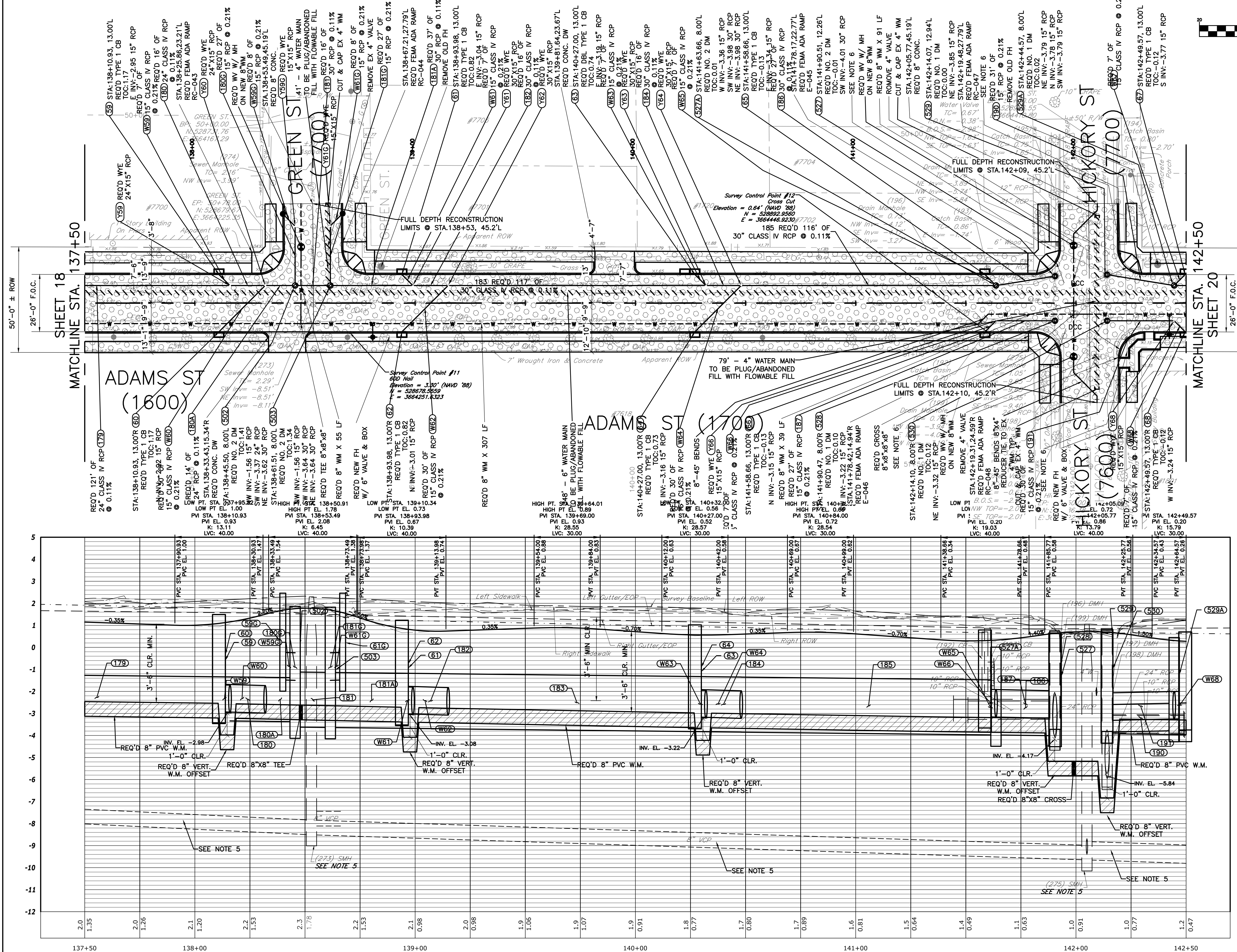
ADAMS STREET (STA: 137+50.00 to STA: 142+50.00) SCALE: 1"=20' HORIZ. / 1"=2' VERT.
