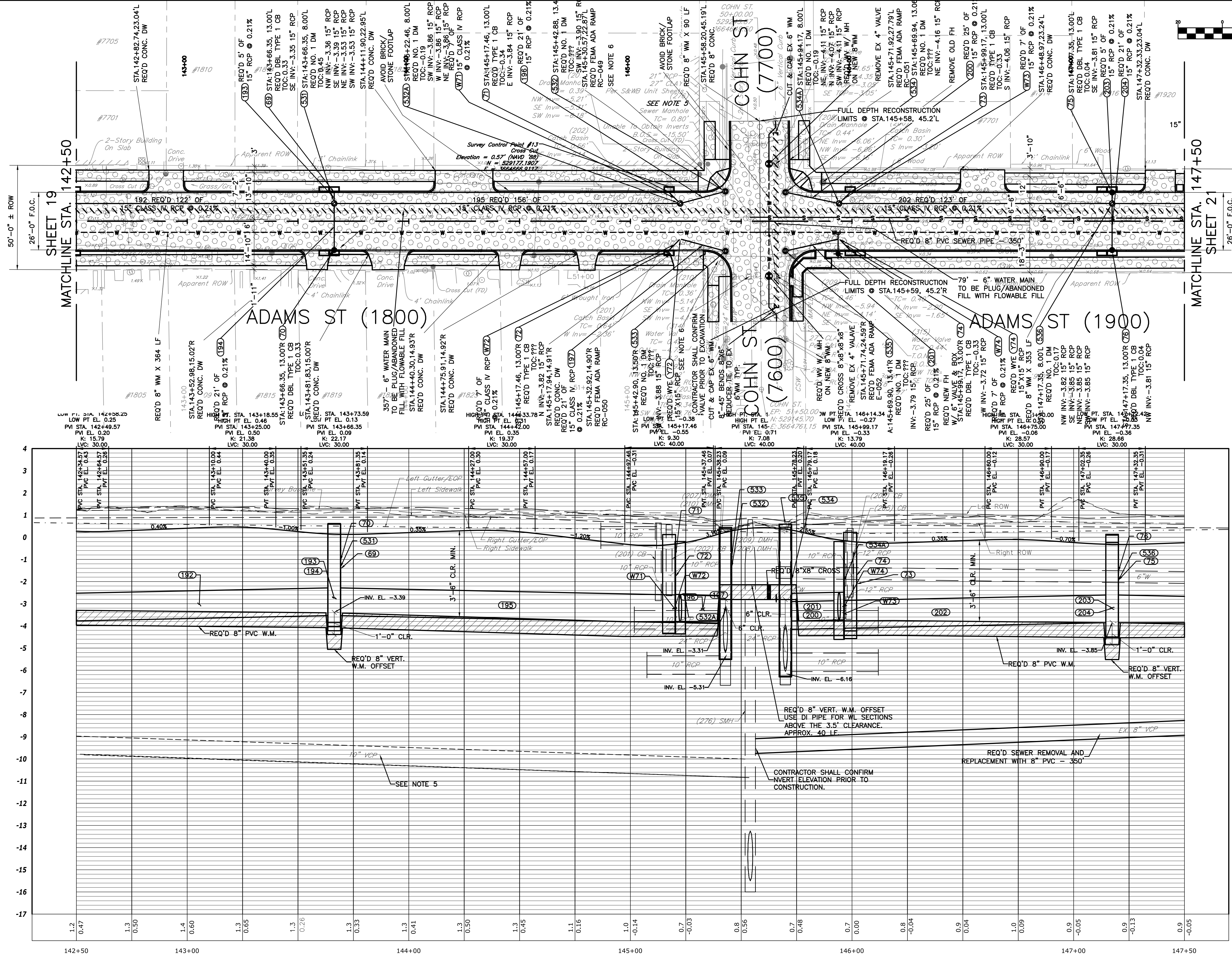
ADAMS STREET (STA: 142+50.00 to STA: 147+50.00) SCALE: 1"=20' HORZ. / 1"=2' VERT.
