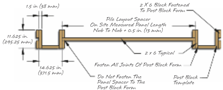
Top View of Panel Block
