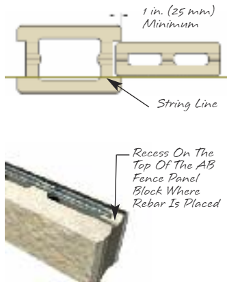
Step 3 Place rebar.
