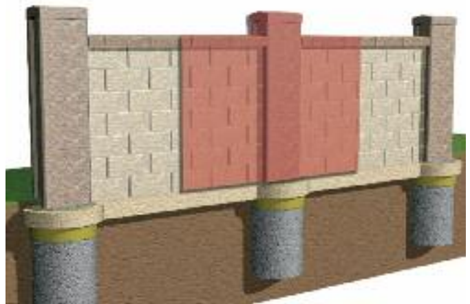
Tributary Area Per Post
