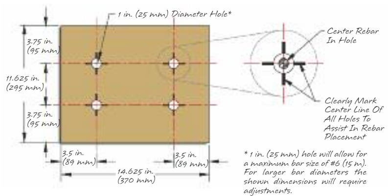
Figure 3: Optional Rebar Alignment Jig
