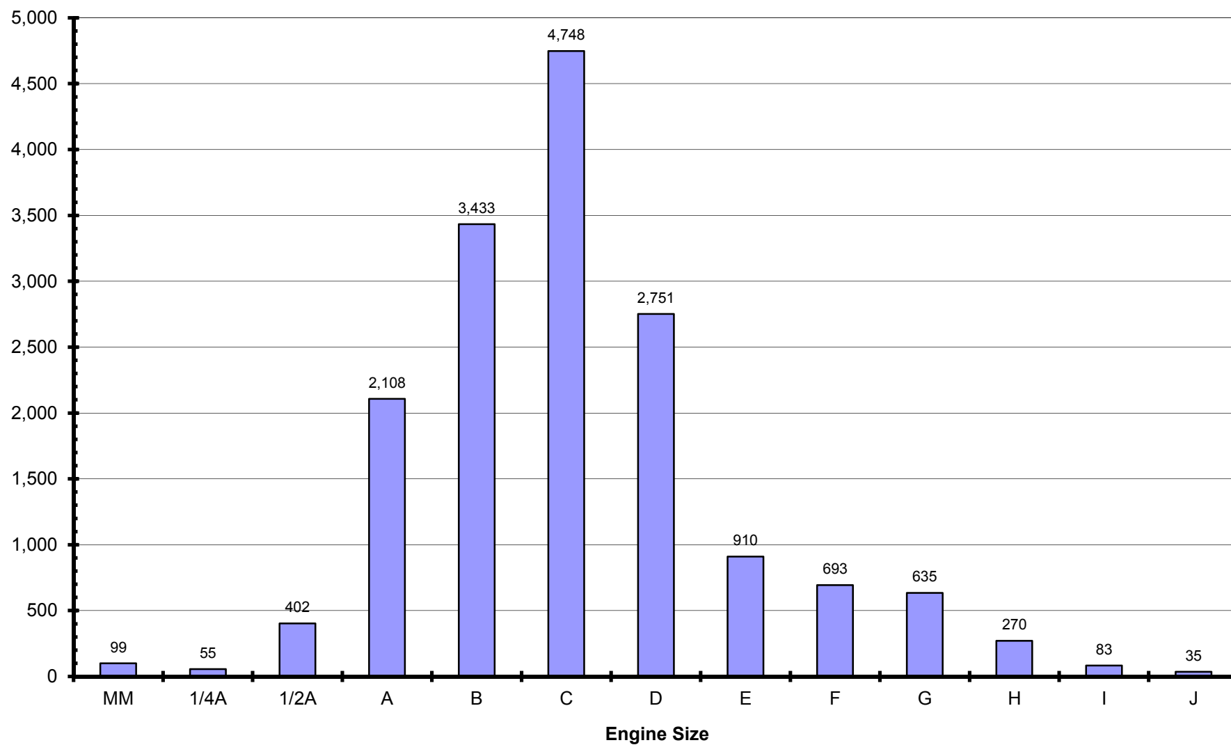
Number of Engines Burned at MASA Launches: 1998 - 2013
