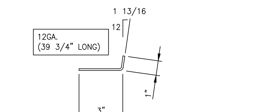
DETAIL OF '14BP12' SCALE: 3"=1'-0"
