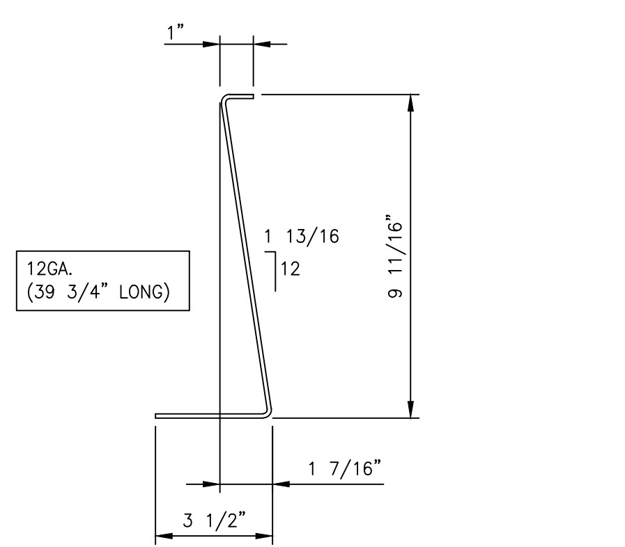
DETAIL OF '14BP11' SCALE: 3"=1'-0"
