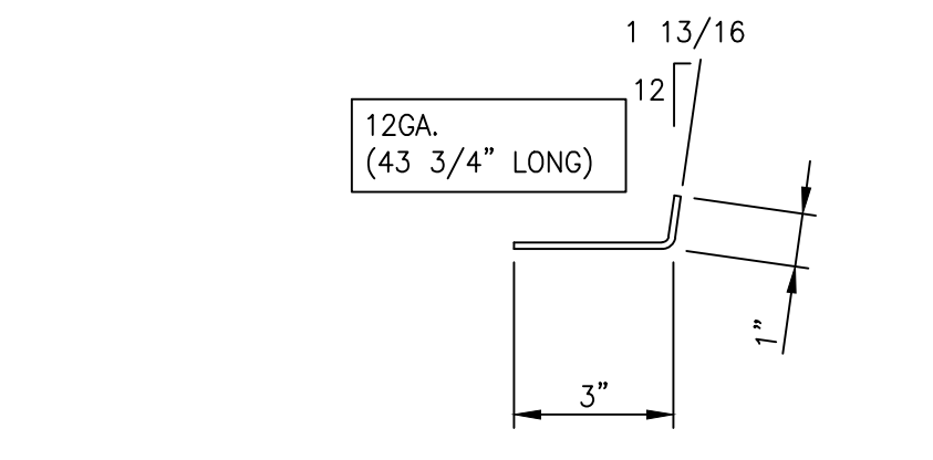
DETAIL OF '14BP3' SCALE: 3"=1'-0"
