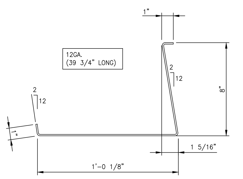
DETAIL OF '14BP4' SCALE: 3"=1'-0"
