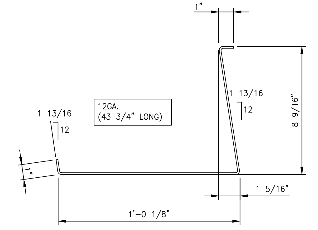
DETAIL OF '14BP1' SCALE: 3"=1'-0"
