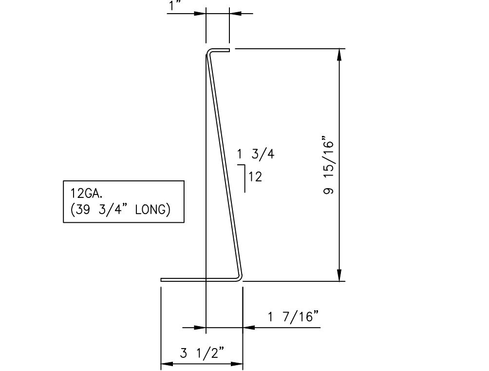
DETAIL OF '14BP8' SCALE: 3"=1'-0"
