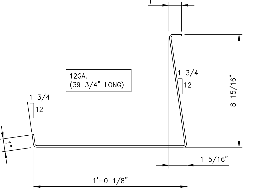
DETAIL OF '14BP7' SCALE: 3"=1'-0"
