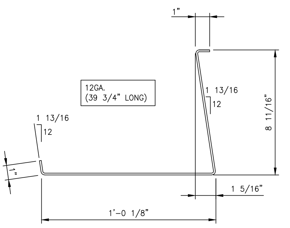
DETAIL OF '14BP10' SCALE: 3"=1'-0"
