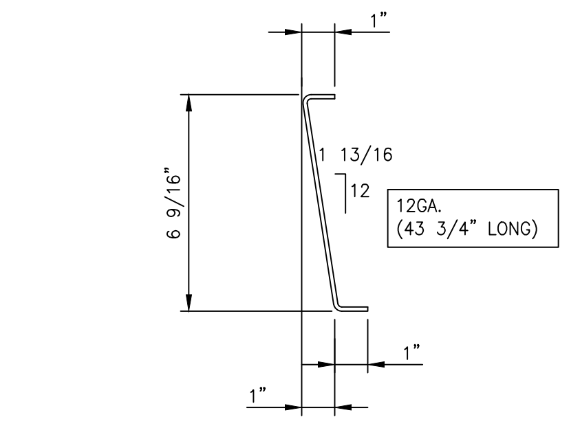
DETAIL OF '14BP2' SCALE: 3"=1'-0"
