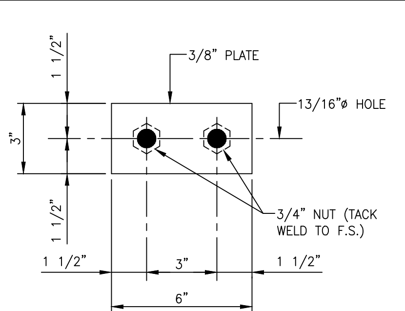
DETAIL OF 'p12' SCALE: 3"=1'-0"
