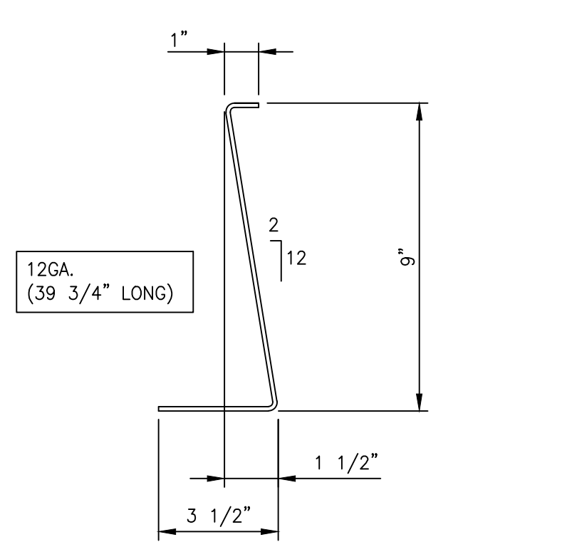
DETAIL OF '14BP5' SCALE: 3"=1'-0"
