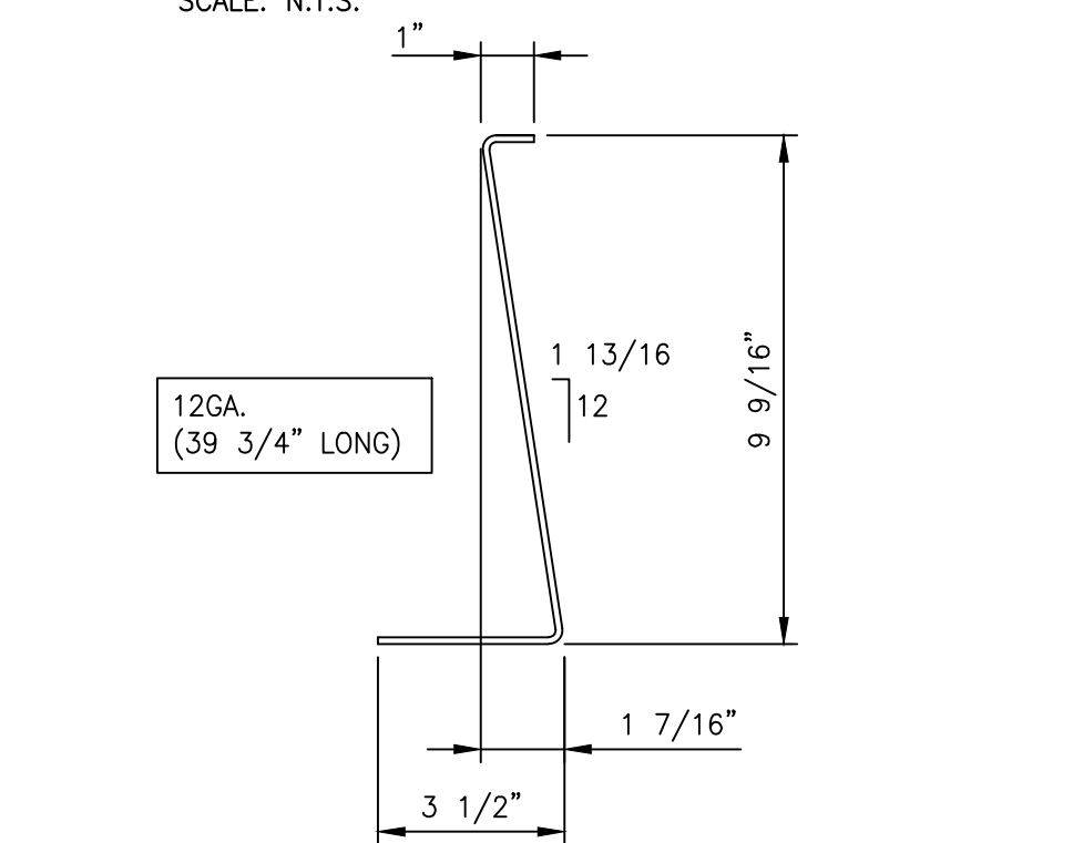
DETAIL OF '14BP13' SCALE: 3"=1'-0"
