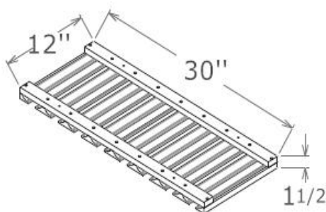
Glass Holder
