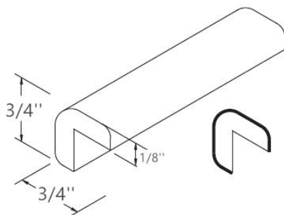
Scribe Moulding
