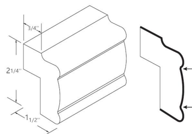
Light Rail Moulding
