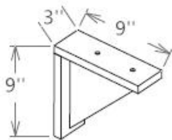
Corbel
