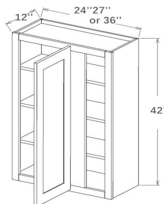
Wall Blind Corner Cabinet, 42" H
