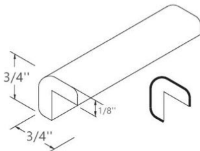
Scribe Moulding
