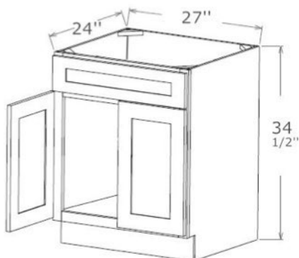
Sink Base
