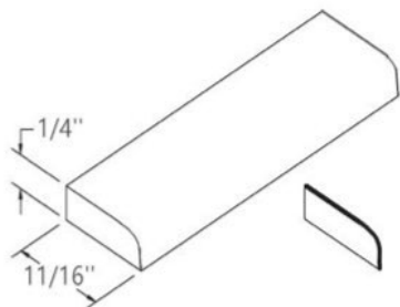
Toe Kick
