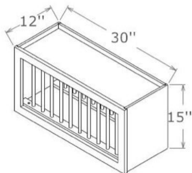
Plate Rack
