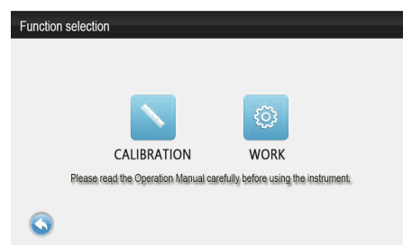
Function Selection
