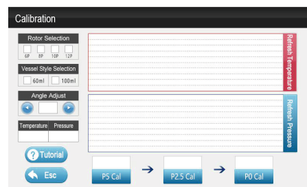
Run Interface
