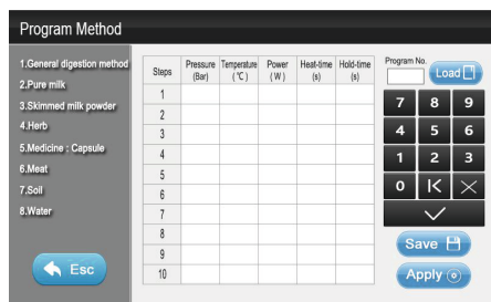
Program Methods
