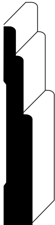
SDW3025 1/2" x 3-1/2"
