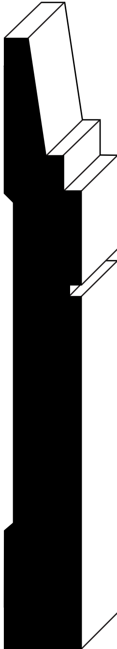
SDW3055 13/16"x 6-1/2"
