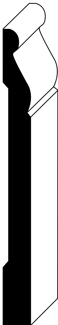
SDW382 1/2" x 5-1/4"
