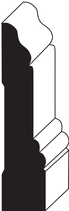
SDW311 3/4" x 3-1/4"
