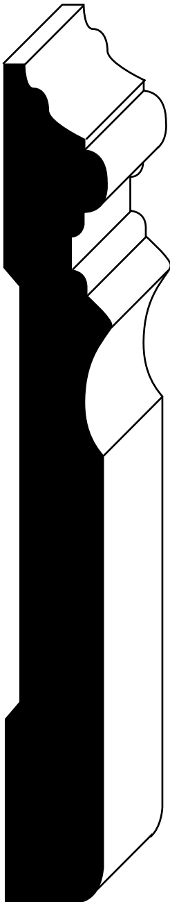
SDW354 13/16" x 6-1/4"
