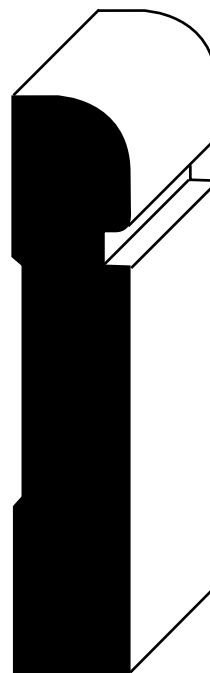
SDW325 5/8" x 3"
