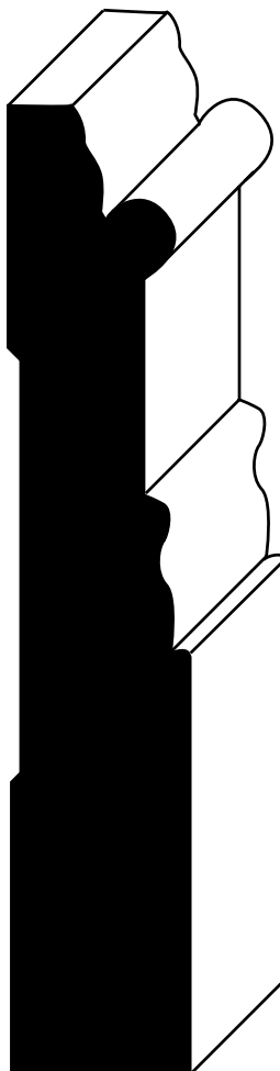
SDW328 13/16" x 4-1/2"
