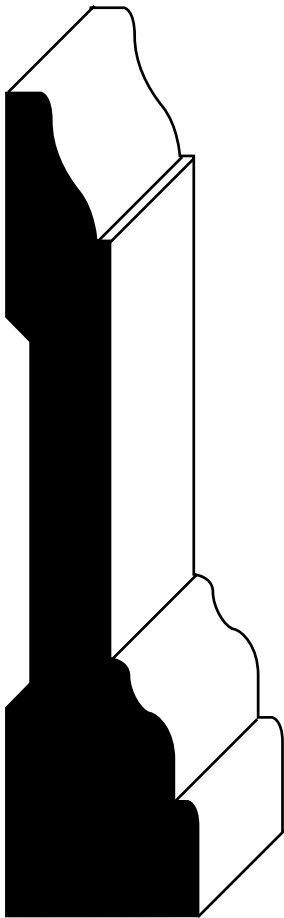
SDW350 1-1/16" x 4-1/4"
