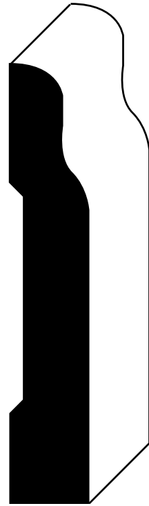
SDW339 1/2" x 3-1/4"
