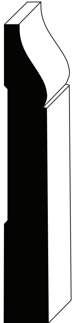
SDW3005 3/4" x 5-1/8"
