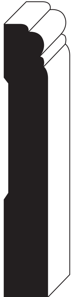
SDW319 3/4" x 4-1/2"
