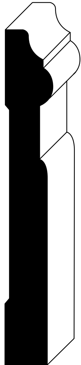
SDW361 13/16" x 5-5/8"
