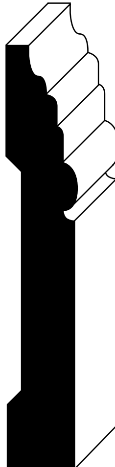
SDW356 11/16" x 4-7/16"
