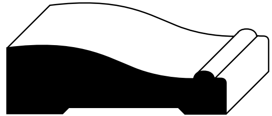
SDW281 11/16" x 2-1/4"
