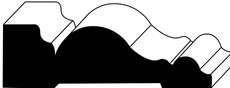
SDW2073 1-1/16" x 3-1/2"
