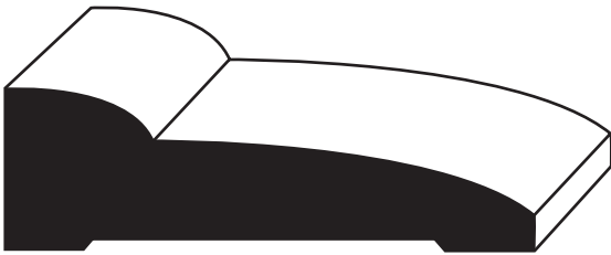
SDW244 3/4" x 2-1/2"
