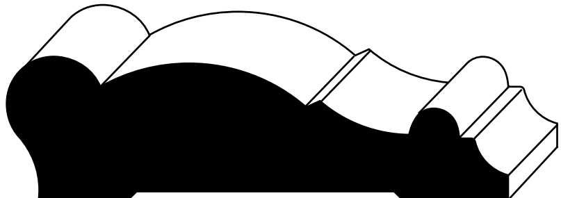
SDW2023 1-1/16" x 3-3/4"
