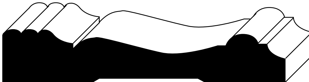
SDW286 13/16" x 4-3/4"
