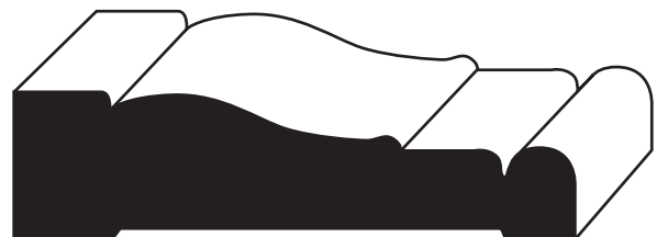
SDW216 3/4" x 2-11/16"
