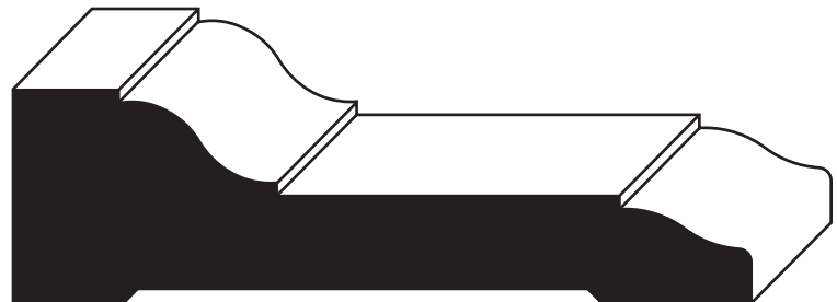
SDW2068 1" x 3-1/2"
