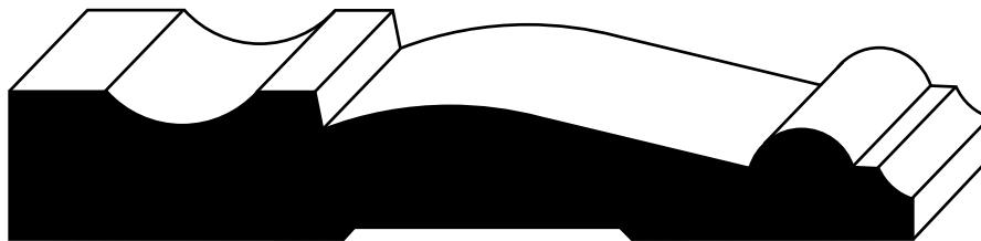
SDW2090 11/16" x 4-1/4"
