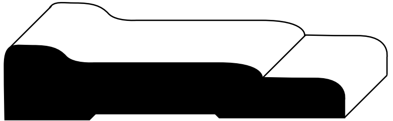
SDW255 3/4" x 3-1/2"
