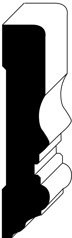
SDW533 13/16" x 4-1/4"
