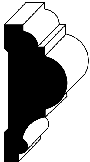
SDW544 1-1/16" x 2-5/16"
