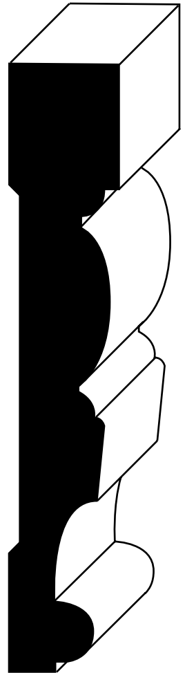
SDW532 13/16" x 4-1/2"
