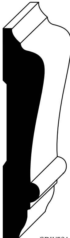
SDW521 3/4" x 3-1/2"
