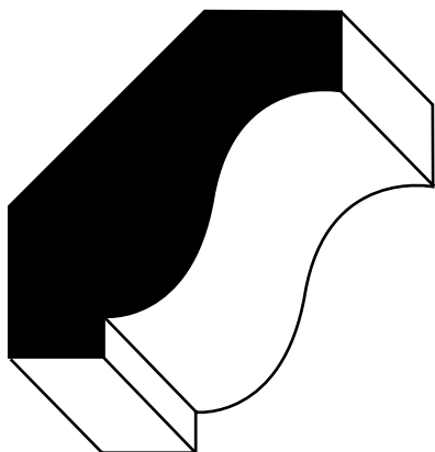
SDW459 13/16" x 2-3/16"
