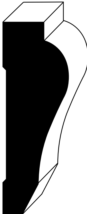
SDW835 1-3/16" x 3-1/2"
