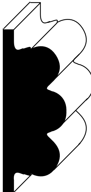
SDW677 1-1/16" x 2-3/4"
