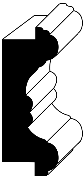
SDW36 Panel Moulding 13/16" x 2-1/2" 1/2 Rabbet
