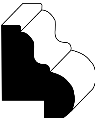
SDW 68 1-1/4" x 1-5/8" with 3/4" Rabbet
