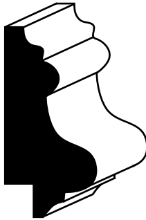
SDW11 Panel Moulding 11/16" x 1-3/8" 1/4 Rabbet
