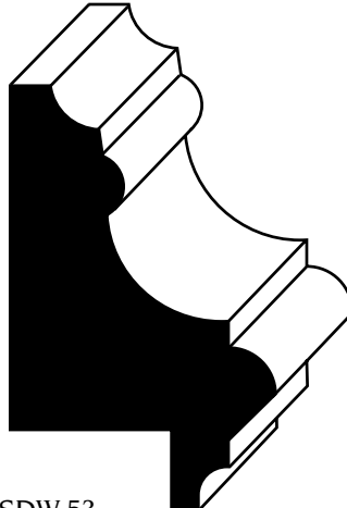
SDW 53 3/4" x 1-1/4"
