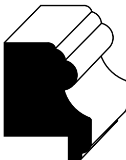
SDW 69 7/8" x 1-3/16"
