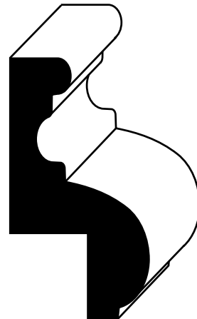
SDW 59 1" x 1-7/8"
