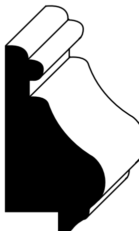
SDW35 15/16" x 2" 1/2 Rabbet
