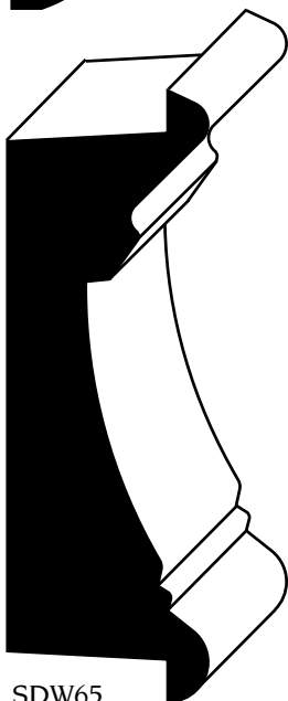
SDW65 15/16" x 2-7/8"
