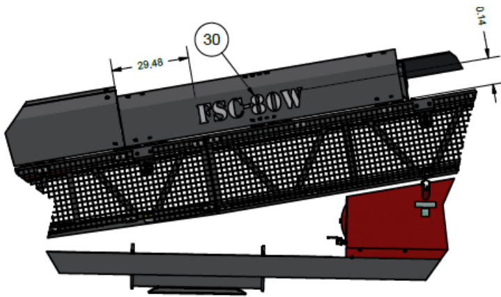
DETAIL G
