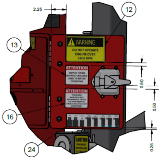
DETAIL L
