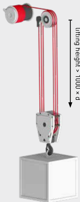
lifting of an unguided load on several falls at a lifting height above 1000 \times d
